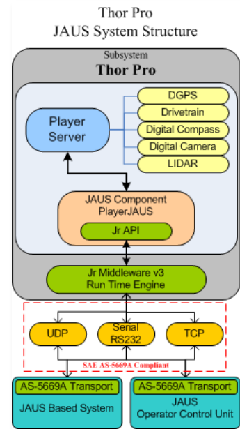
Figure 12: Thor Pro JAUS Structure
