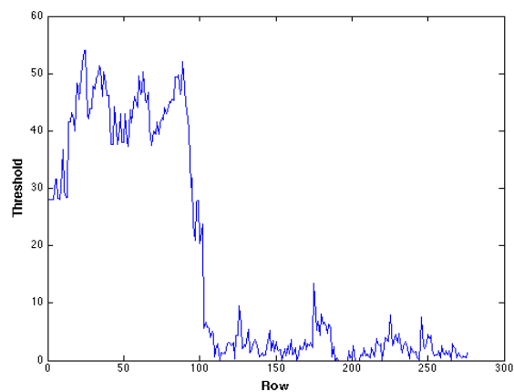
Figure 8: Adaptive Thresholding
